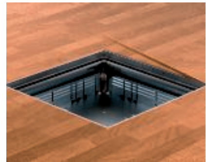
Laying the floor covering on the cassette frames RKS Seal the remaining gap between the floor covering and the cassette frame with suitable materials (possibly with a cork strip).
