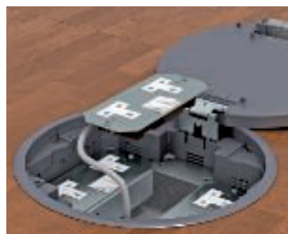
Device mounting Connect device and fix it together with cover plate in mounting tray.
