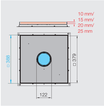
RKF 2, for tube body, nominal size 350-3
