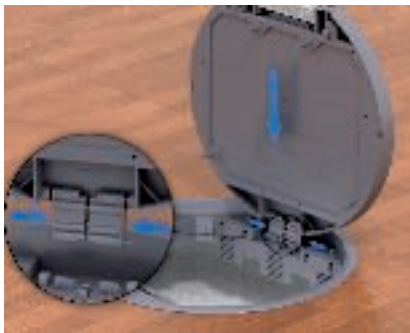
Insertion of the hinged lid Push the hinge together and insert in the holder in the frame.
