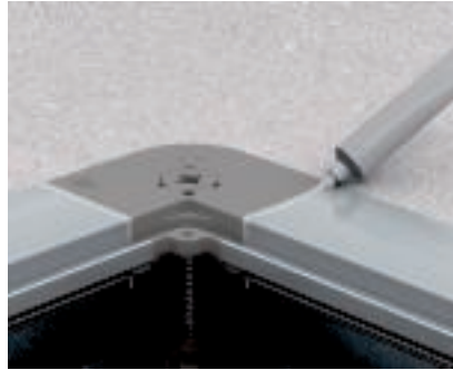
Sealing of the cassette frame with silicone (only RK and RKF) Seal the frame of the underfloor box in the corners using silicone (silicone is included in the scope of delivery of the cassette).
