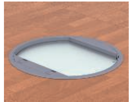
Adjust of the floor covering recess to 10 mm Slacken the 4 lid screws and the inserted 7 mm spacer frame and replace it with the 2 mm spacer bars. Screw the sheet steel lid on again.
