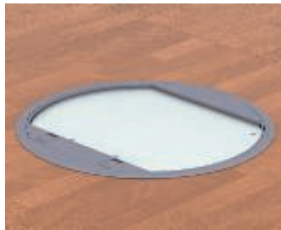
Installation of the hinged cover for GESR round service outlet Slacken the 4 lid screws and the inserted 7 mm spacer frame and replace it with the 2 mm spacer bars. Screw the sheet steel lid on again.
